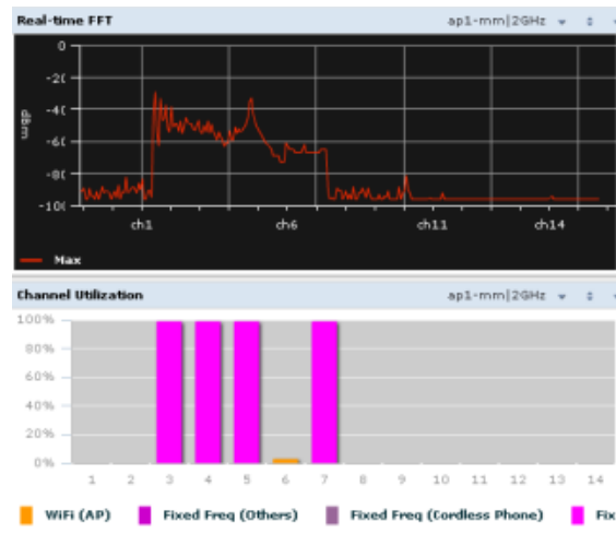
Figure 11: Channel Utilization During Outside Signal Generation
