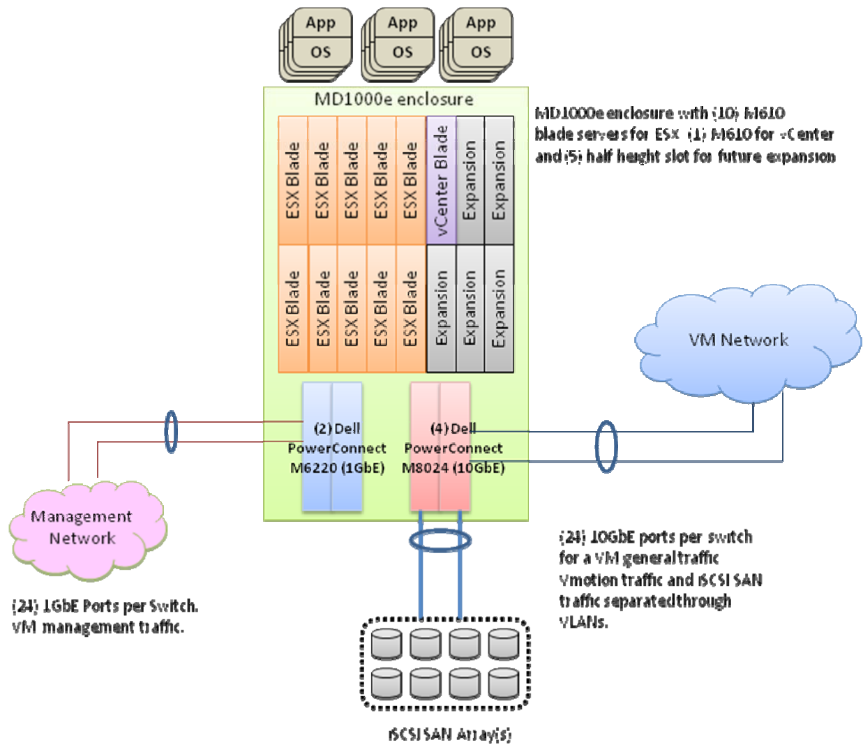
Figure 2: Typical virtualization deployment
